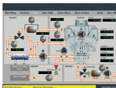
„Health Care“ for the Engine: Highest durability through secured and monitored lube oil supply.
