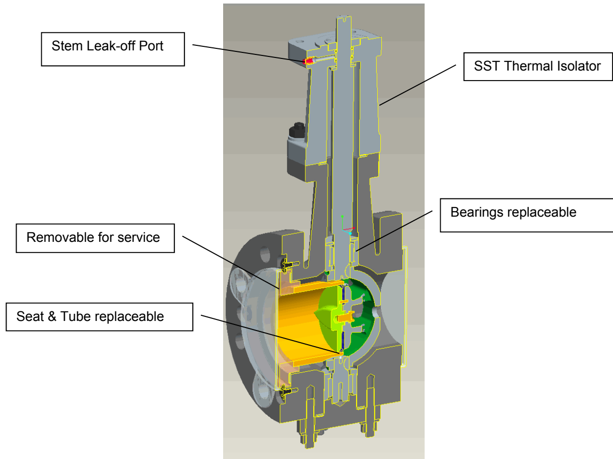
RVP-200 Cutaway Drawing
