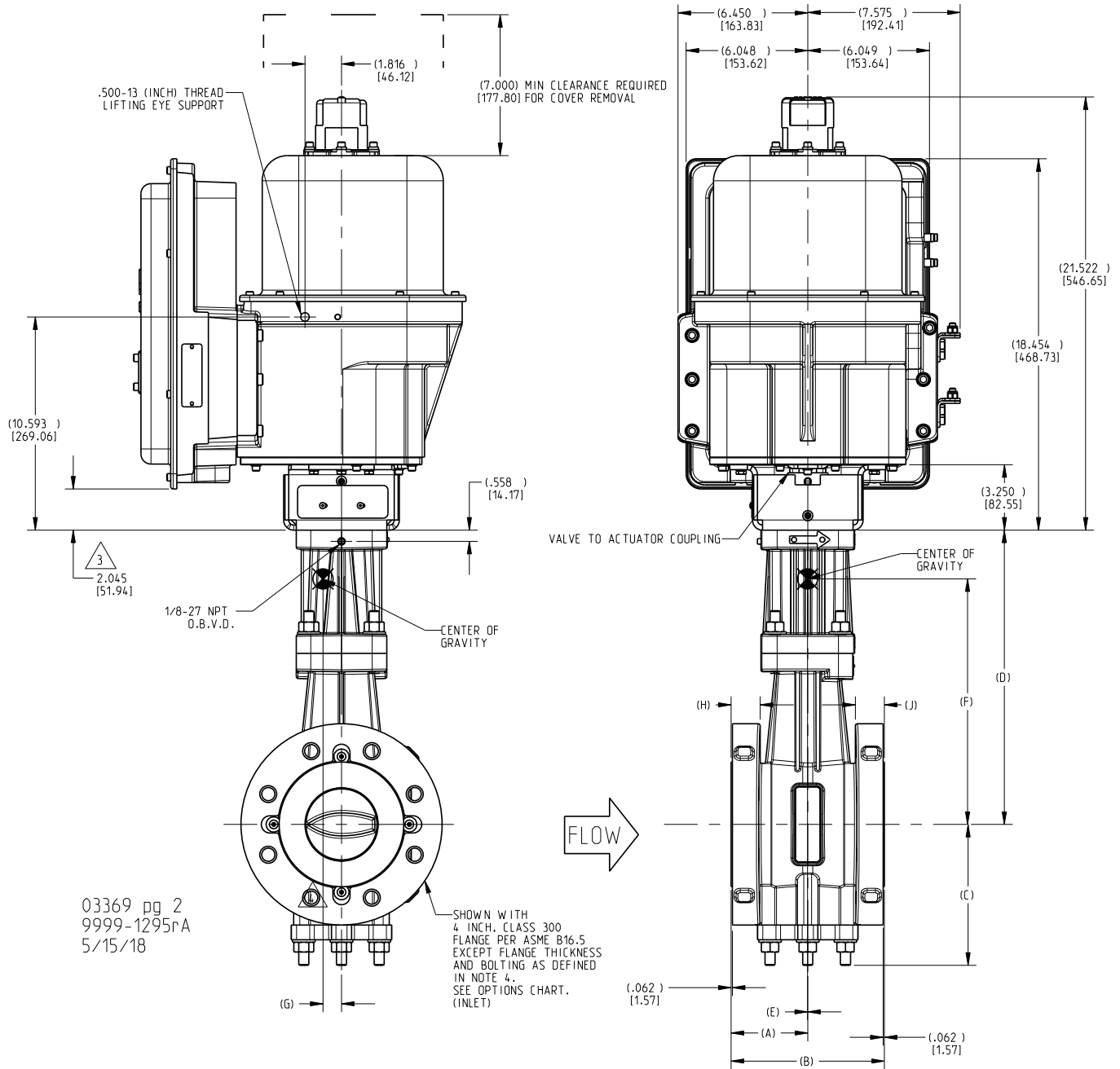
RVP-200 Outline Drawing (inches) [mm]
