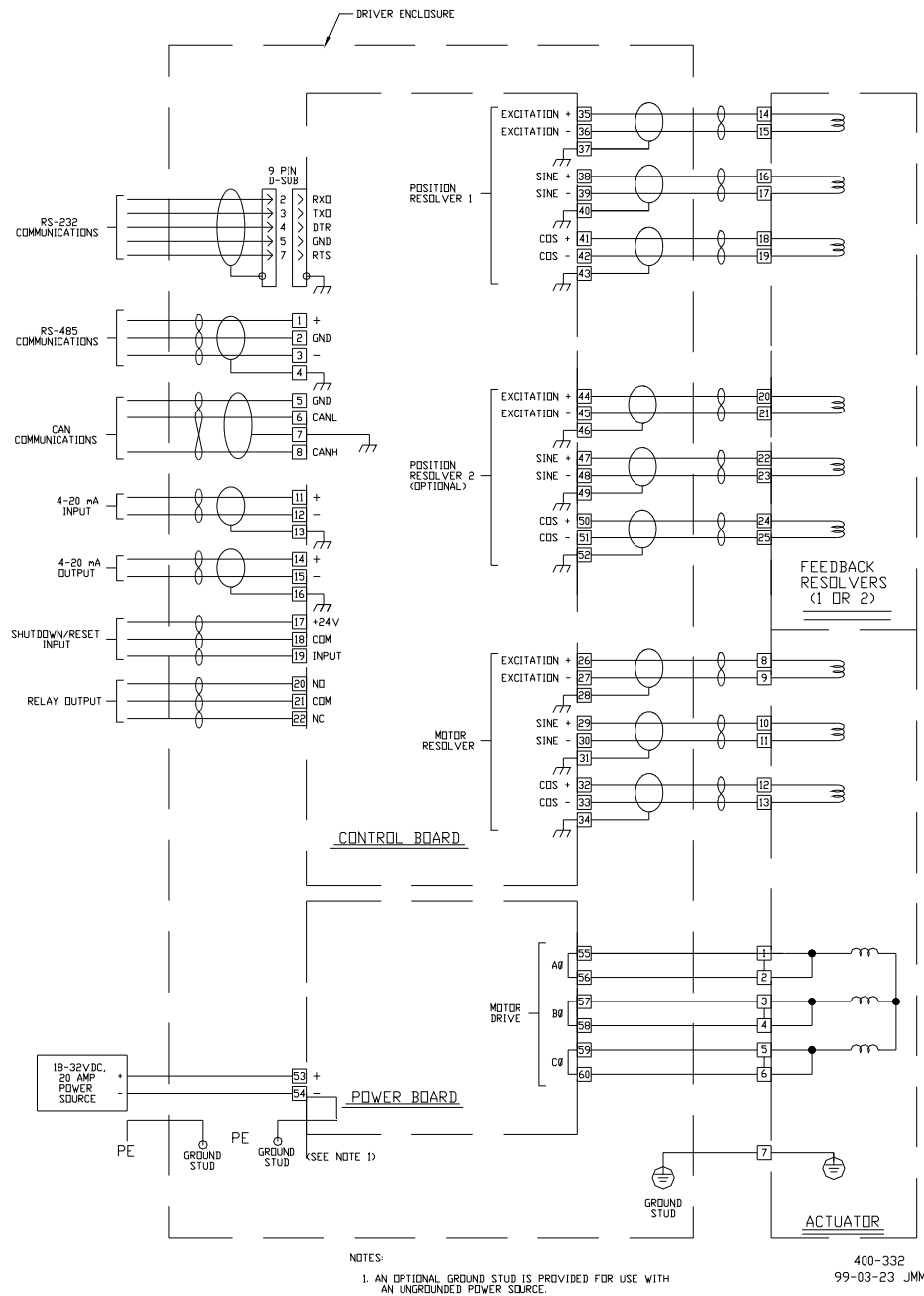
Wiring Diagram (EM Driver shown)
